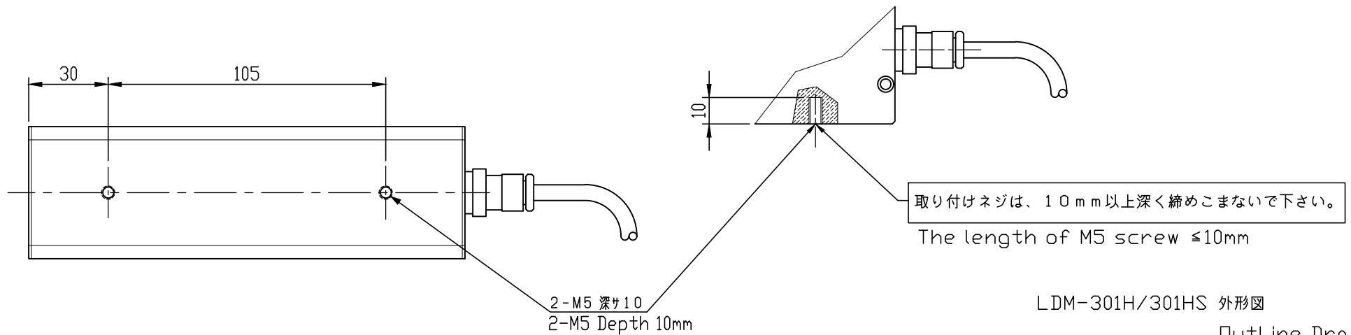
Outline Drawing
